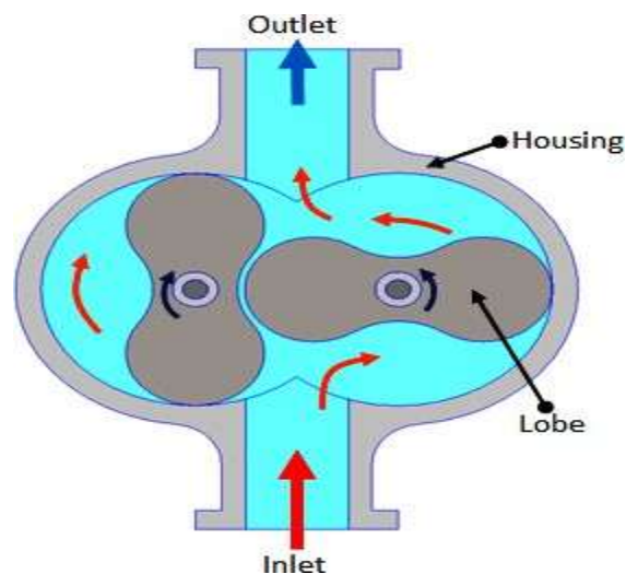
Fig- Lobe pump
