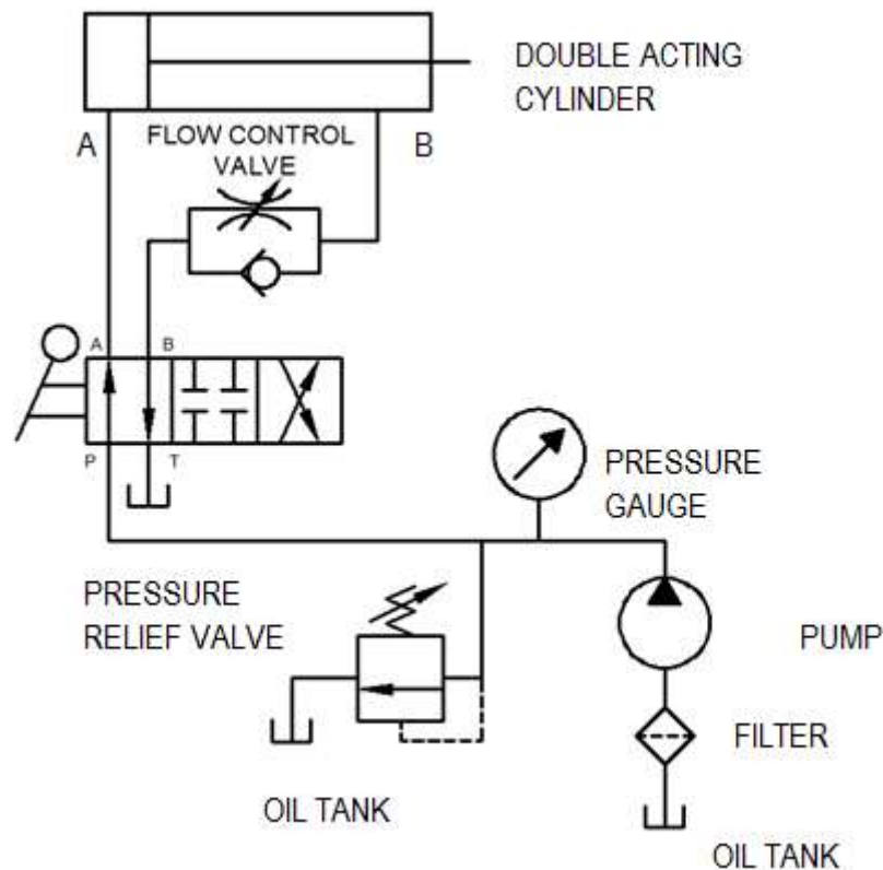
Fig - Meter out speed control circuit
