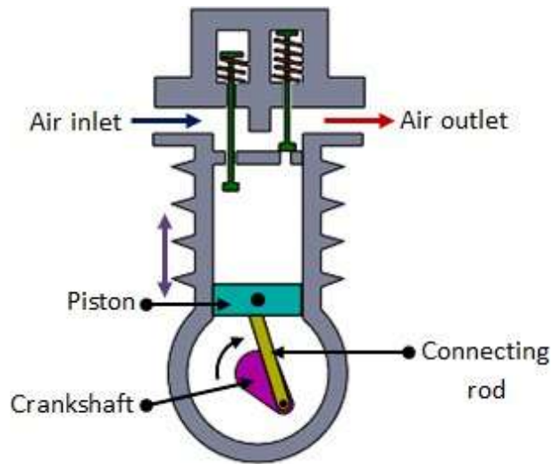
Fig- Piston compressors
