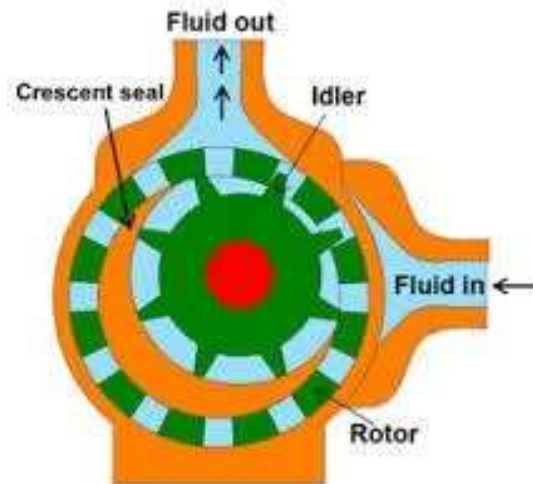
FIG-INTERNAL GEAR PUMP
