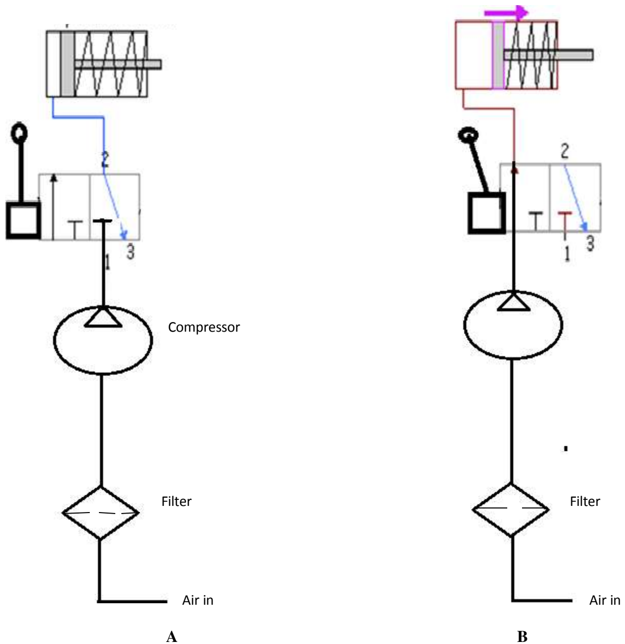
Fig- Working of single acting cylinder operation
