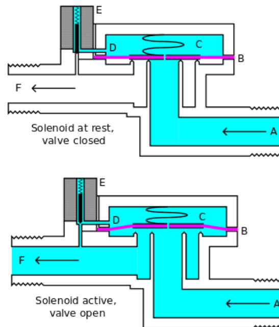
Fig- working of Solenoid valve
