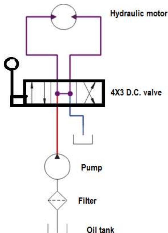
Fig- Working of double acting cylinder and hydraulic motor
