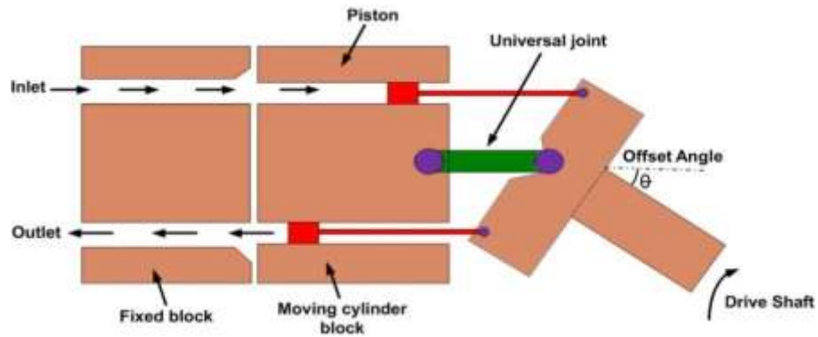
Fig- Bent axis piston pump
