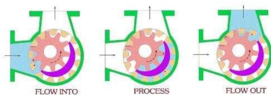
FIG- WORKING OF INTERNAL GEAR PUMP
