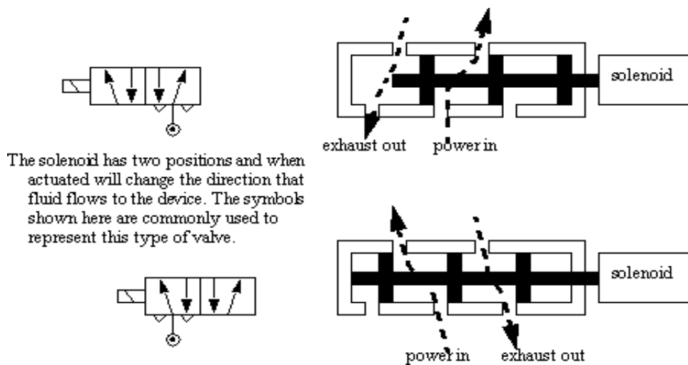
Fig- Working of Solenoid valve
