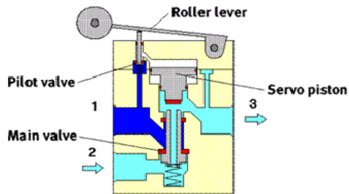
Fig- Working of limit switches
