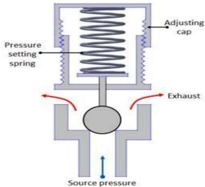
Fig.-Rotary relief valve
