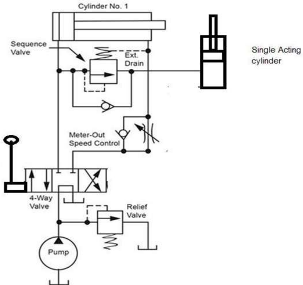
Fig. Working Sequencing circuit
