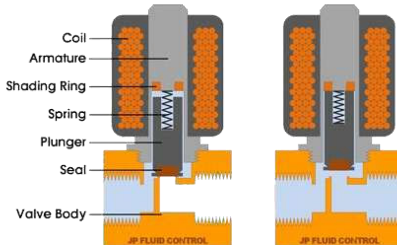
Fig. direct acting solenoid valve
