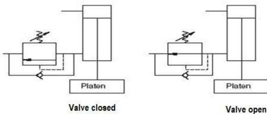
Fig –Working circuit of Counterbalance
