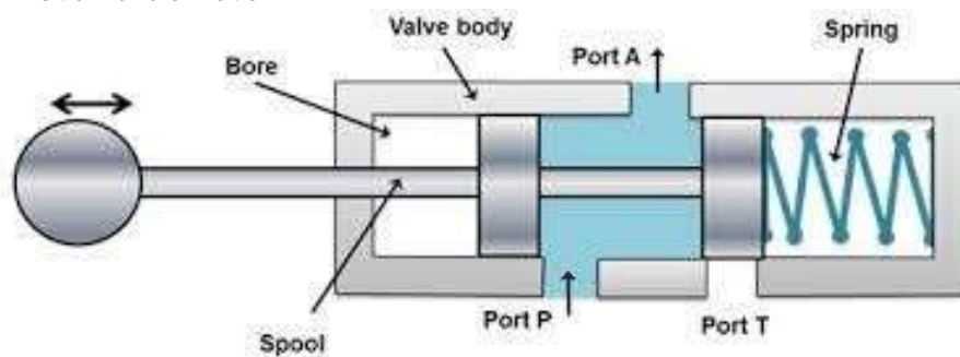
Fig-Manually operated 3X2 D.C. valve
