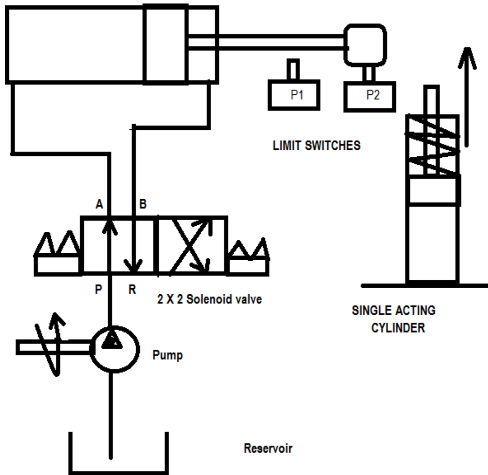
Fig- Working of Solenoid valve
