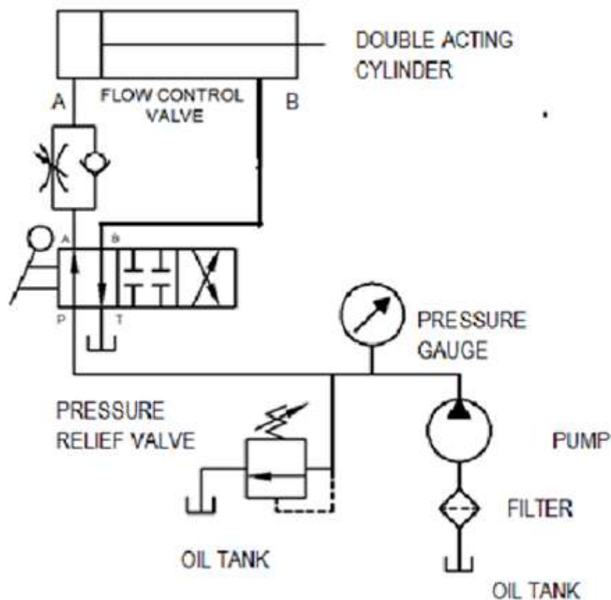
Fig Meter in speed control circuit
