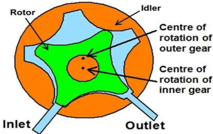
Fig- Working of gerotor pump
