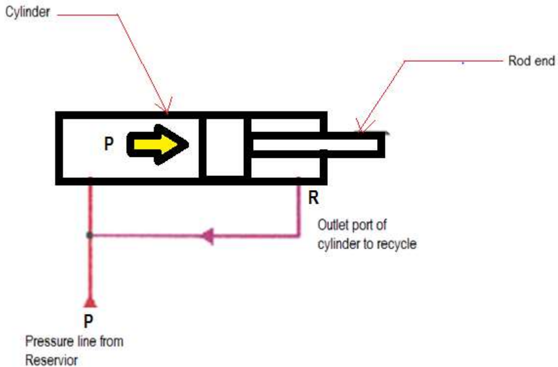
Fig: Connection of a regenerative
