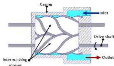
Fig- Screw compressor
