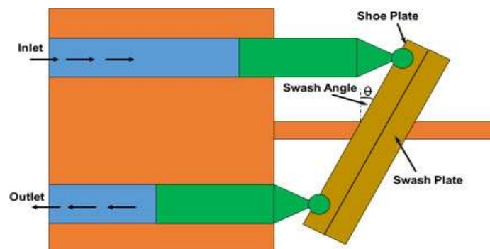
Fig- Swash Plate Piston Pump
