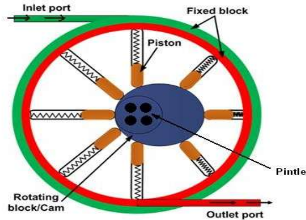
Fig- Radial piston pump
