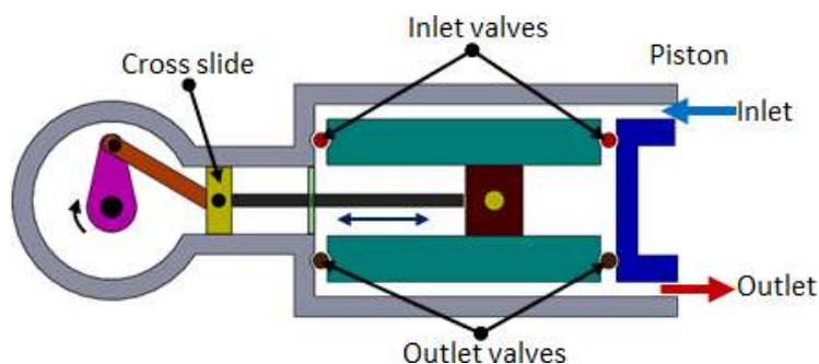
Fig- Double acting compressor
