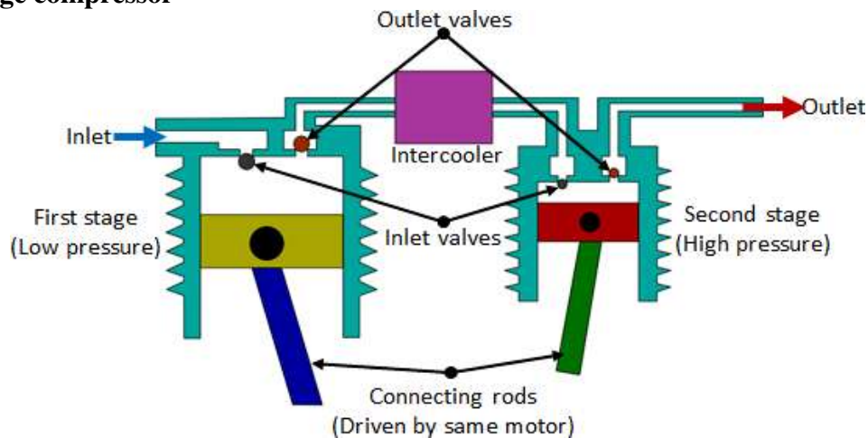
Fig-Multistage compressor
