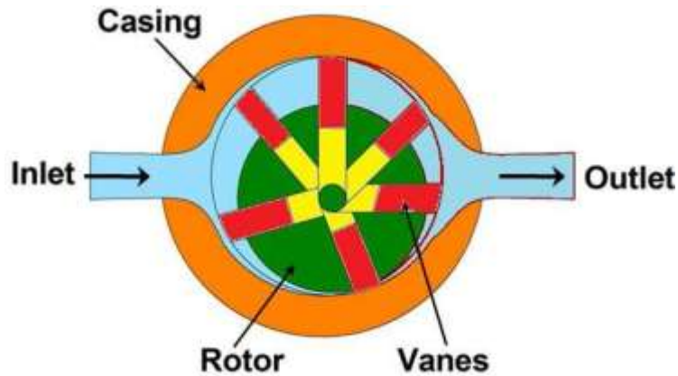
Fig- Vane compressor
