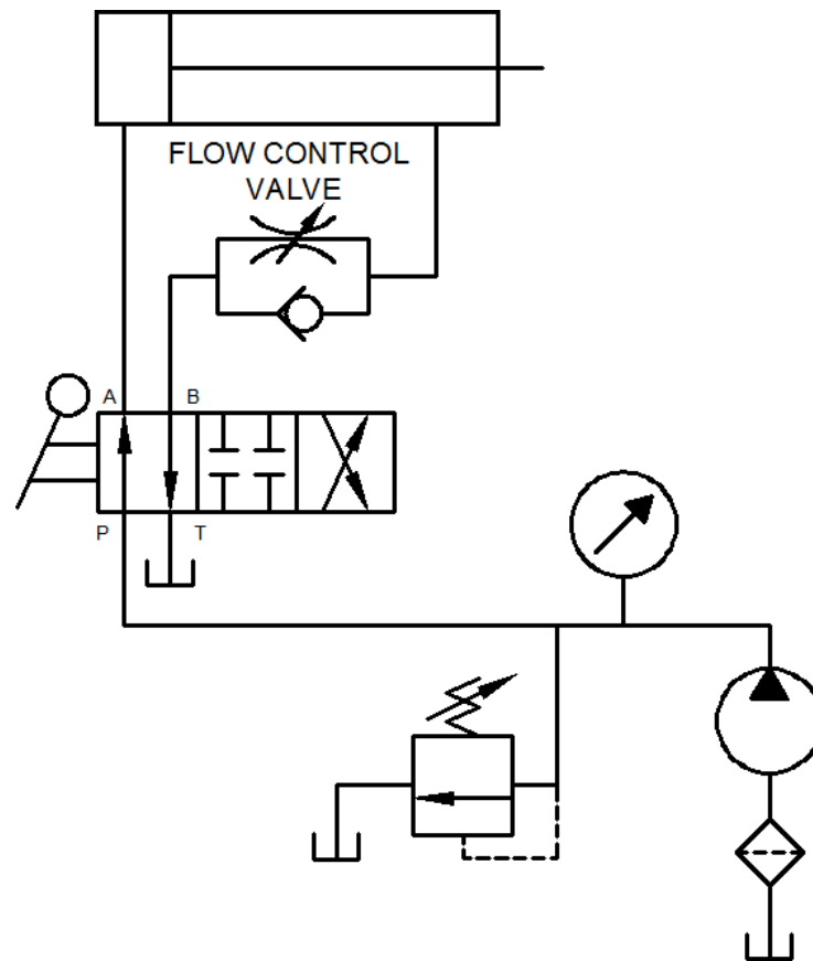
Fig. Meter out circuit for shaping machine
