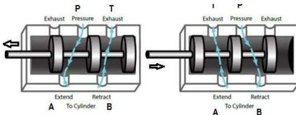
Fig: Spool type 5x2 Valve
