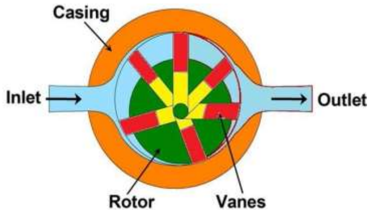
Fig : Unbalanced Vane pump
