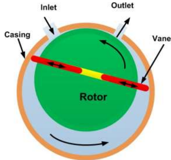
Fig- Vane pump
