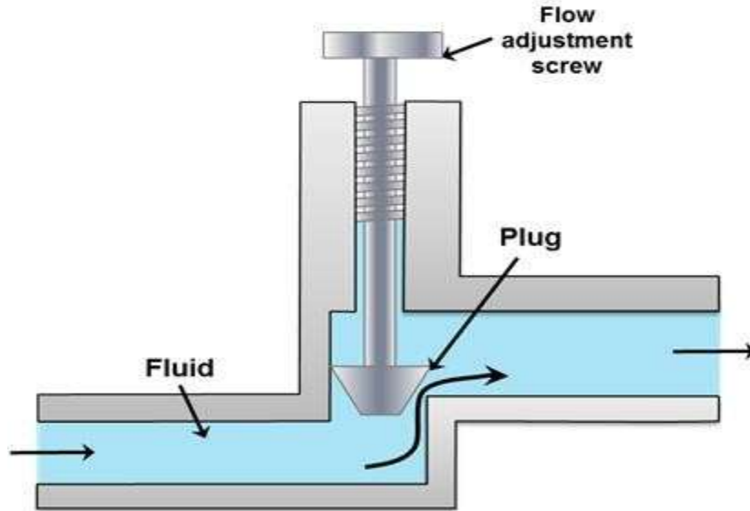
Fig- Flow control valve
