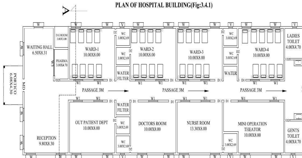
PLAN OF HOSPITAL BUILDING(Fig:3.4.1)
