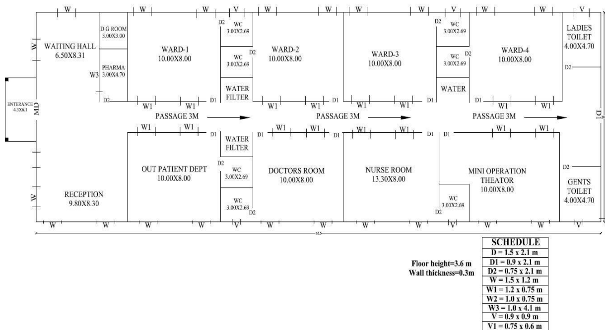
Q.no.3.4:-LINE DIAGRAM OF HOSPITAL BUILDING
