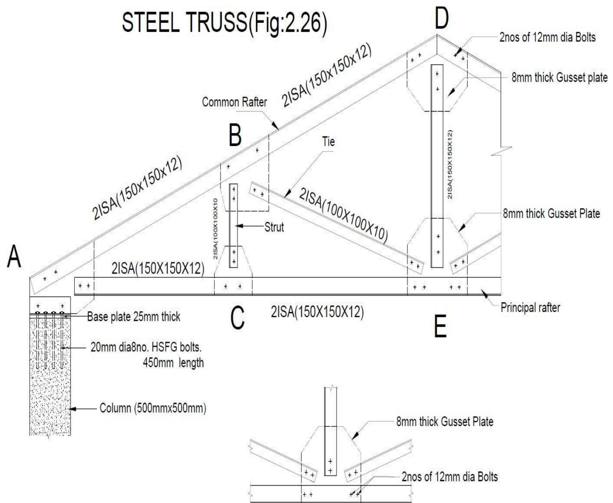
Detail at E
